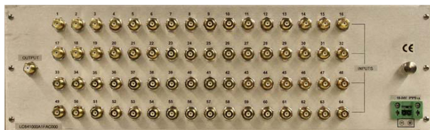
LC64 1000A 64-way Active Broadband Combiner
