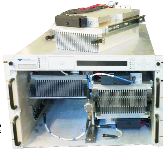
Hot-swappable SSPA Modules
