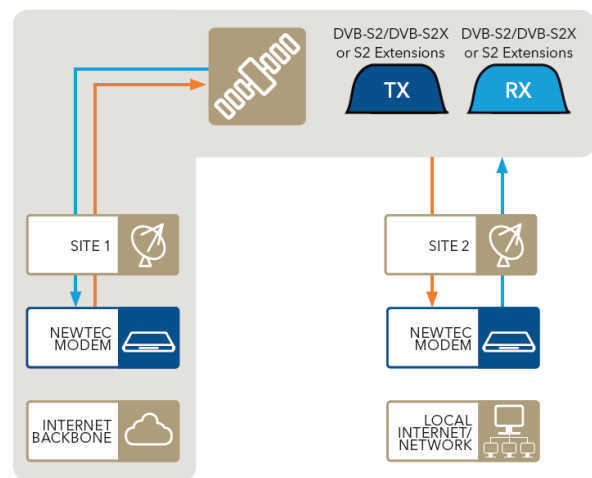
Point-to-point
