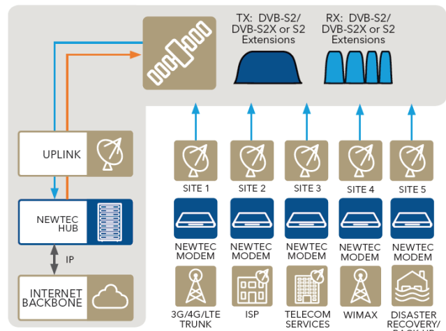
Point-to-multipoint
