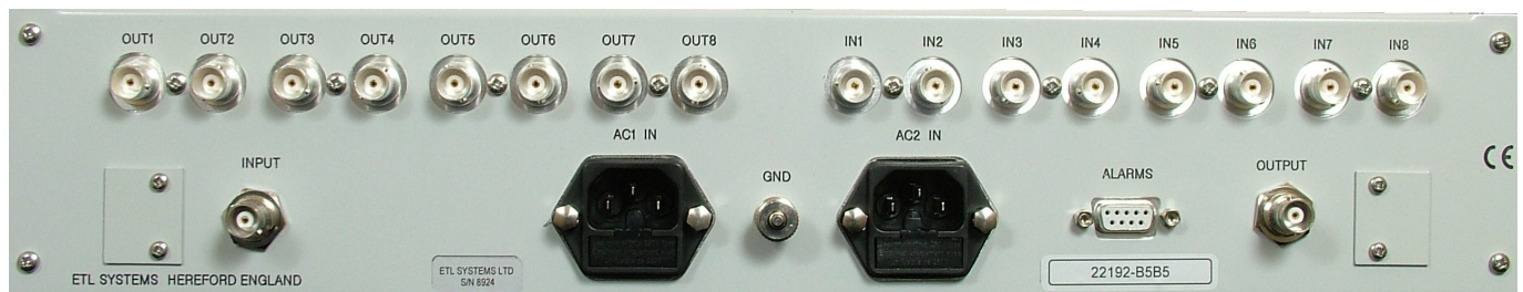
Rear View of Model 22192 with 50 ohm BNC connectors
