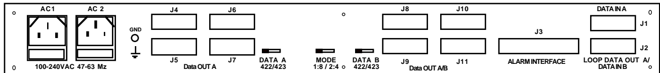
FIGURE 2.0 1583-10 Rear Panel
