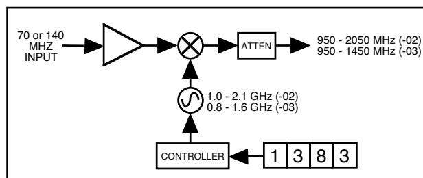
Block Diagram
