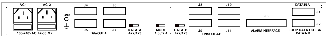
FIGURE 2.0 1583-10 Rear Panel
