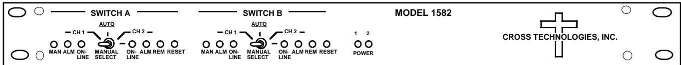
1582-16 Front Panel
