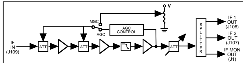
Block Diagram
